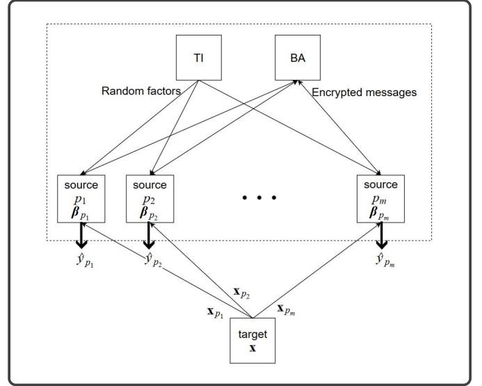
Fig. 2. Inference phase of privacy-preserving target-independent LR.
