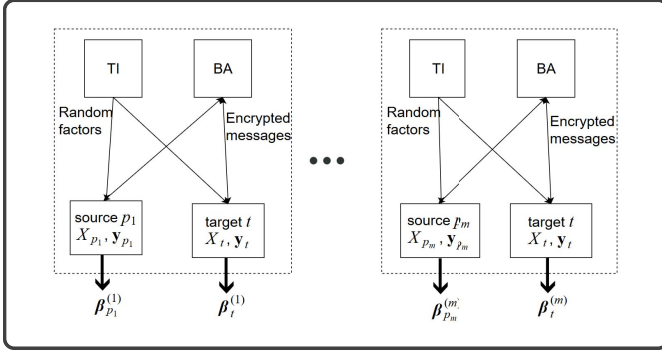
Fig. 3. Training phase of privacy-preserving target-calibrated LR.
