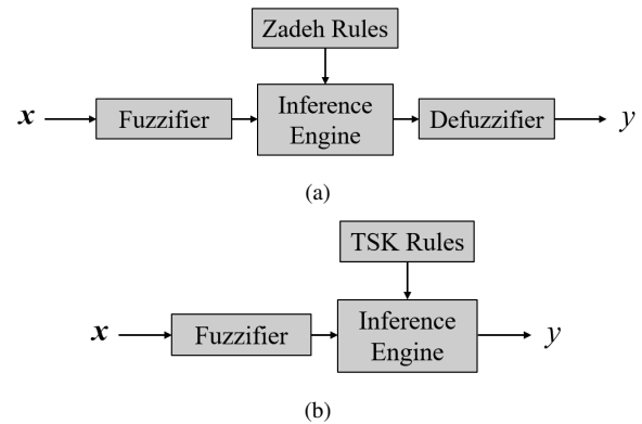
Fig. 1. (a) Flowchart of a Zadeh (Mamdani) fuzzy system; (b) flowchart of a TSK fuzzy system.
