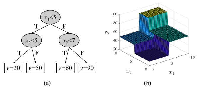
Fig. 5. (a) An example of CART for regression; and, (b) its input-output mapping.
