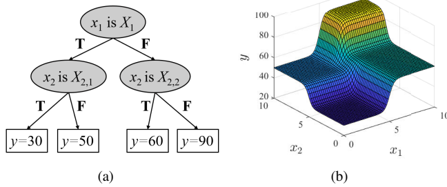
Fig. 6. (a) An example of fuzzy CART for regression; and, (b) its input-output mapping.
